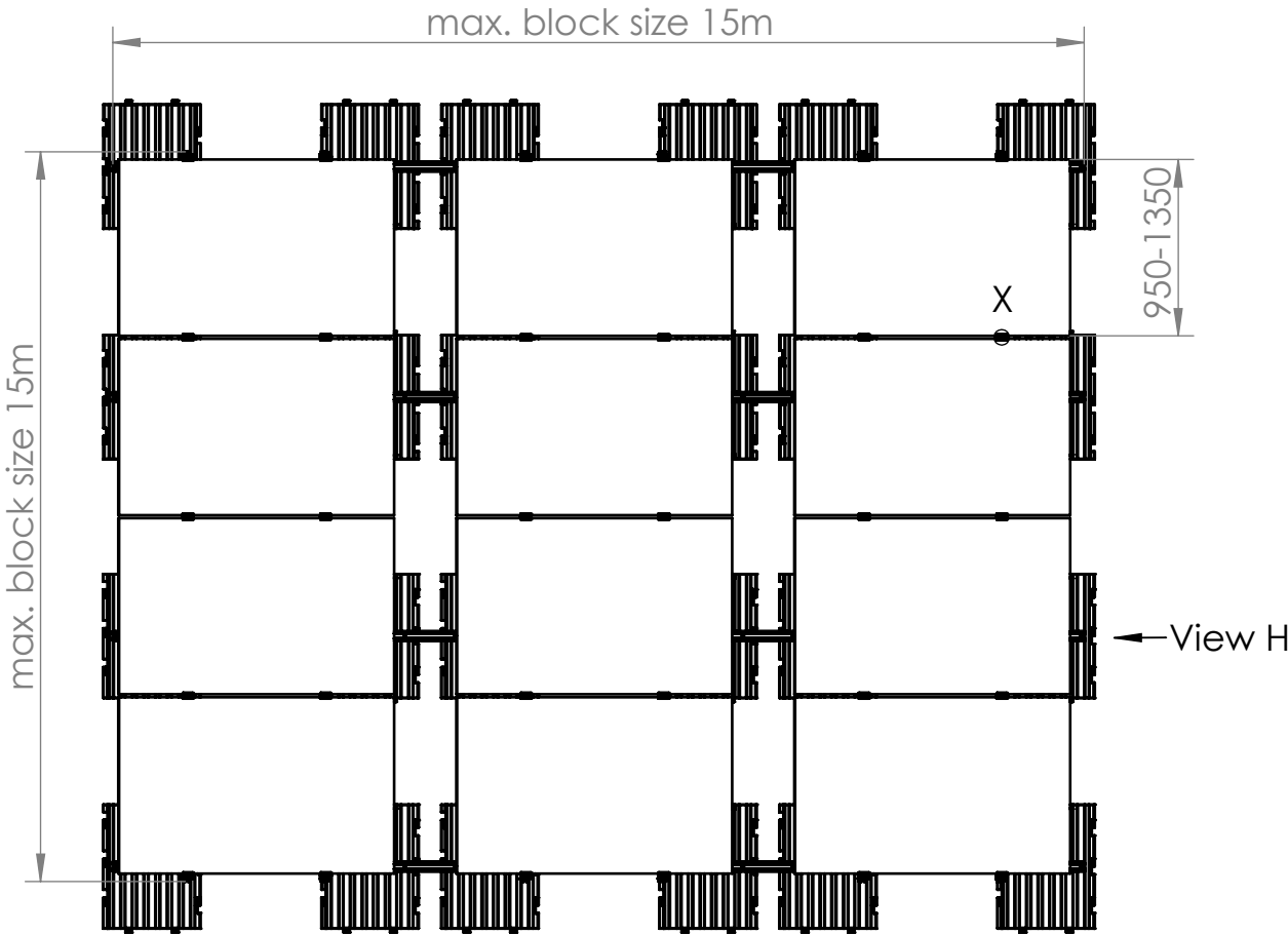
Plan view 1 : 50
